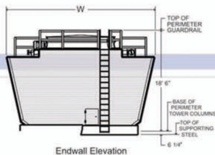
Endwall Elevation
